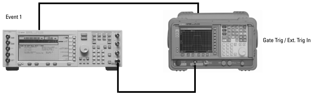
Figure 2. An ESG-D series signal generator (left) connected to an ESA-E series spectrum analyzer (right).
