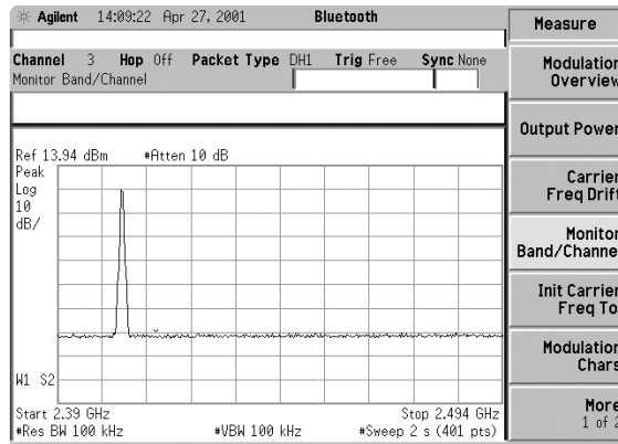
Figure 9. Monitor/band channel measurement under measure menu. The input signal stays at one channel.
