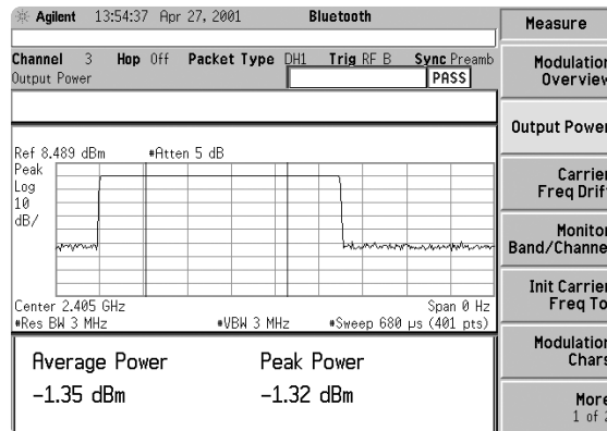
Figure 3. Output power measurement under measure menu.
