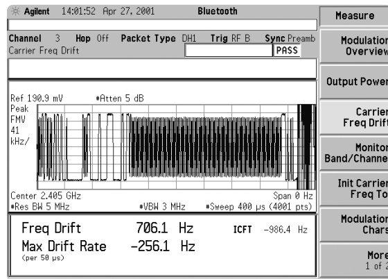
Figure 7. Carrier frequency drift measurement under measure menu.
