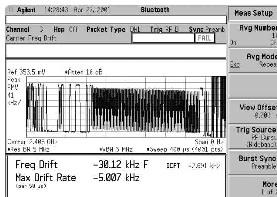
Figure 8. Measurement setup menu for carrier frequency drift.
